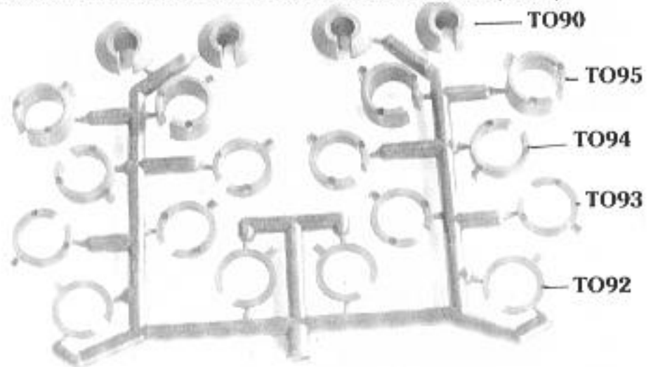
T613 SPRING STOPS & SPACERS MOULDING (T511)
