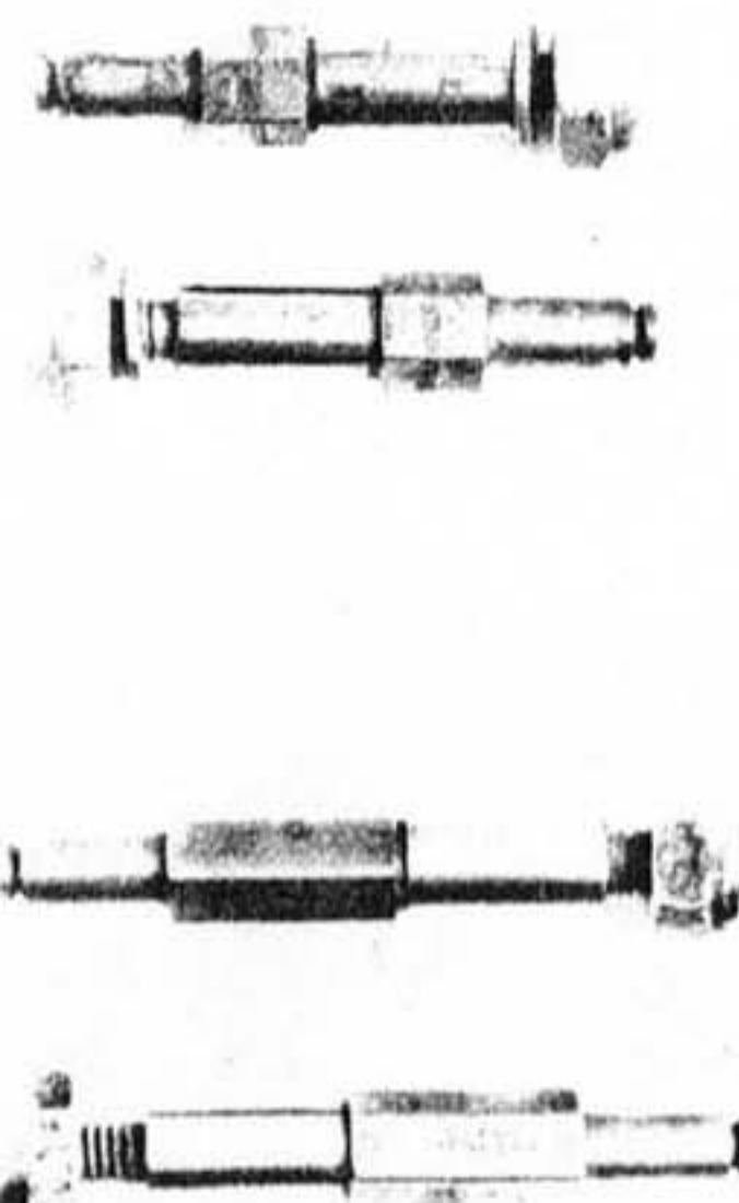
1552/1553/1557 - STUB AXLES - Our direct replacement RC10 front stub axles are hardened and ground to meet racing standards. All have larger leads to reduce breakage and have a T shape to fit Associated steering blocks without modification. 1552 - RC10 FRONT STUB AXLES FOR TAMIYA BEARINGS $8.99 1553 - RC10 FRONT STUB AXLES FOR ASSOCIATED BEARINGS $8.99 1557 - RC10 FRONT STUB AXLES - WIDE TRACK FOR TAMIYA BEARINGS $8.99
