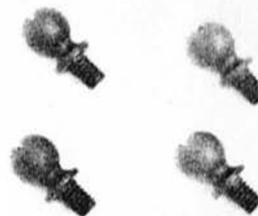
1551 - FRONT SUSPENSION PIVOT BALLS - Replaces aluminum 8mm ball connectors with heavy-duty steel balls, reducing chance of wear and breakage. Designed for steering blocks with larger thread holes. 4 pieces. Fits Hot Shot, Super Shot, Big Wig, Boomerang, HSII, and Super Sabre. $6.99
