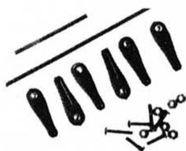
1501 - HEAVY-DUTY "STOCK" STEERING - Special heim joint ends coupled with 4-40 stainless steel rod eliminates those troublesome ball joints and weak steering rods. Replaces all three rods. Complete with all screws and nuts. Tamiya RR, SS, F-150, SC. $6.99
